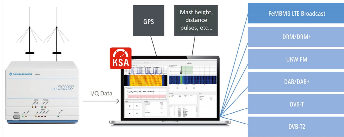
picture: Principle and illustration Kathrein Signal Analyzer "KSA"
